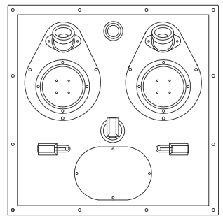
Duplex Unit Square Pit
