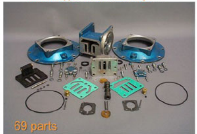
Warren Rupp 2" Air Distribution System
